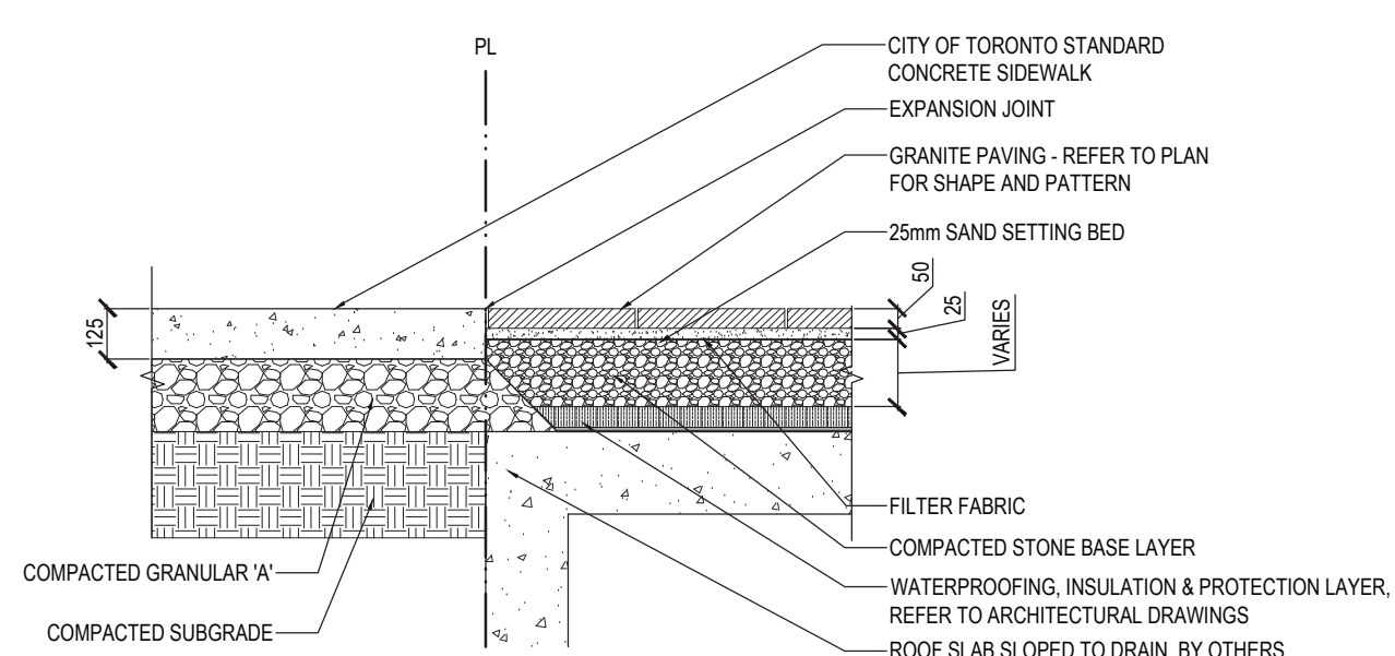
5 PAVING DETAIL ON/OFF SLAB SCALE=1:20
