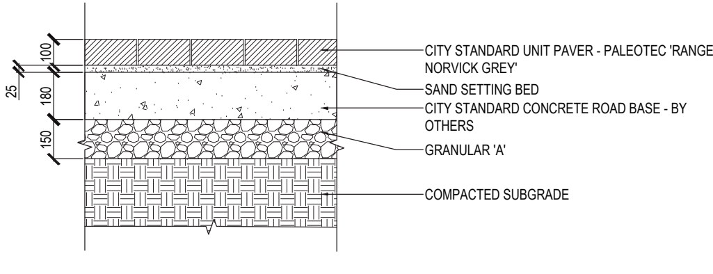
6 CITY STANDARD VEHICULAR UNIT PAVER SCALE=1:20
