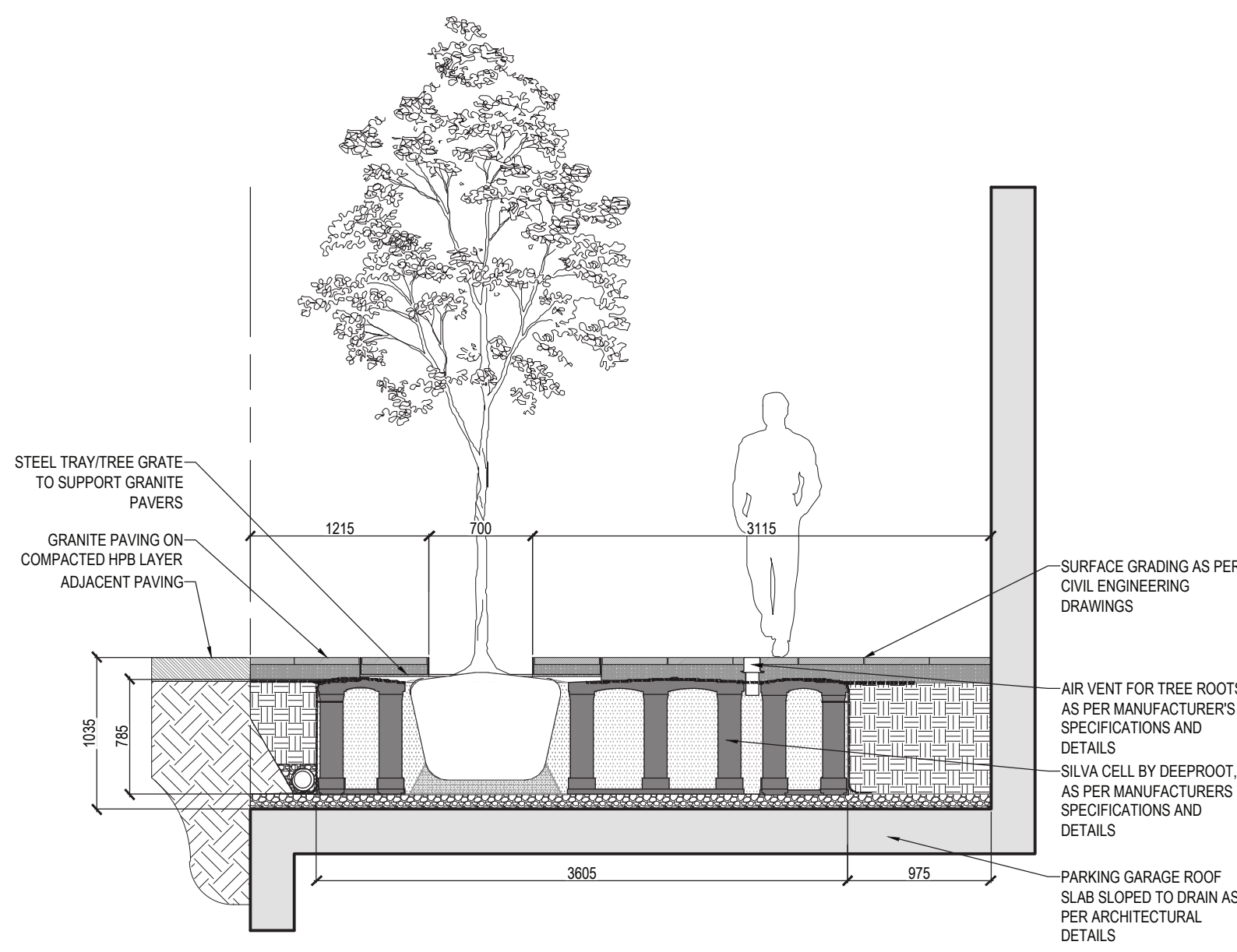
8 SOIL CELL SECTION SCALE=1:40
