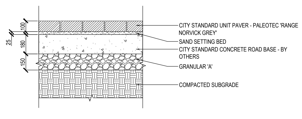
6 CITY STANDARD VEHICULAR UNIT PAVER SCALE=1:20
