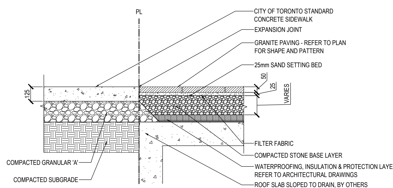
5 PAVING DETAIL ON/OFF SLAB SCALE=1:20
